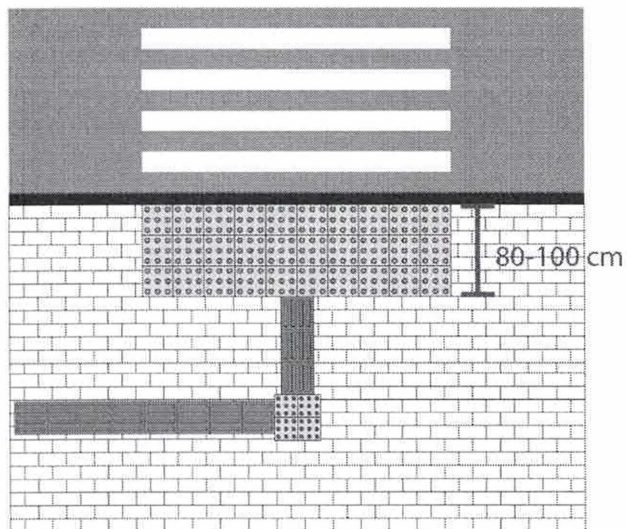
WARIANT 1
